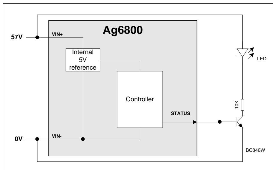
The Ag6800 STATUS output pin has a limited drive capability. This is sufficient to drive a logic input, but does not have enough power to continually drive an LED. Figure 12 shows a simple circuit to drive an LED from the STATUS output. Over driving the STATUS output can result in damage to the internal 5V reference supply.
