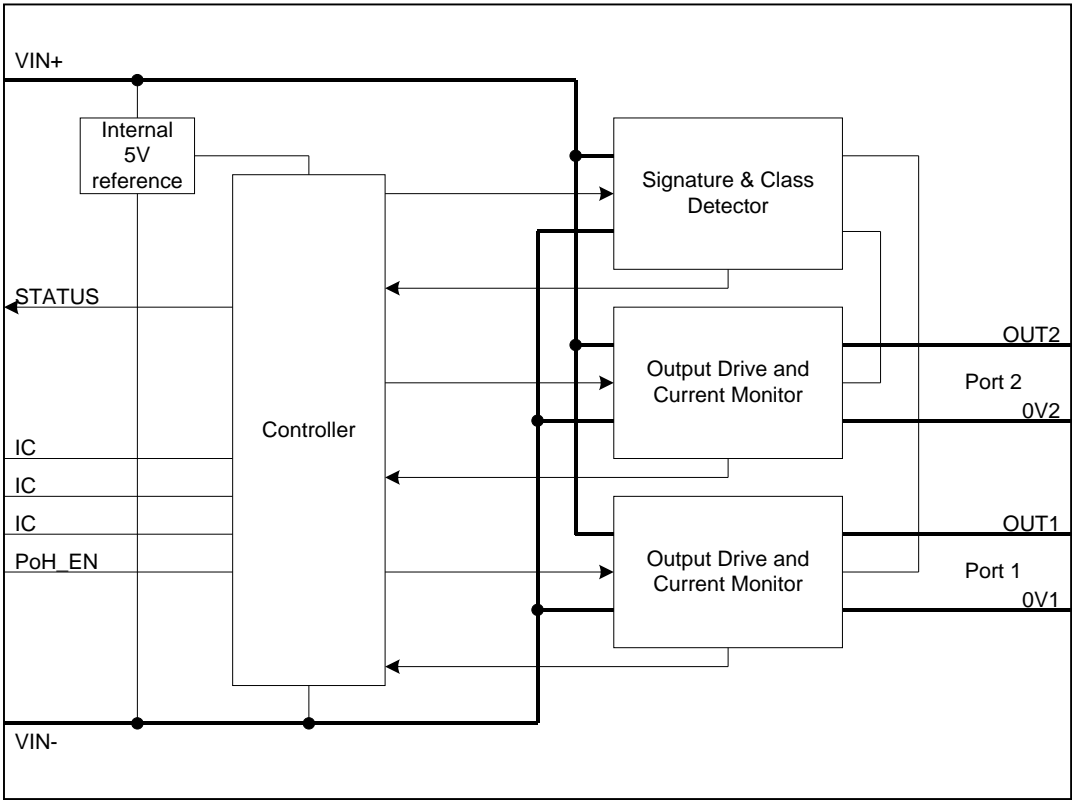
Figure 1: Block Diagram
